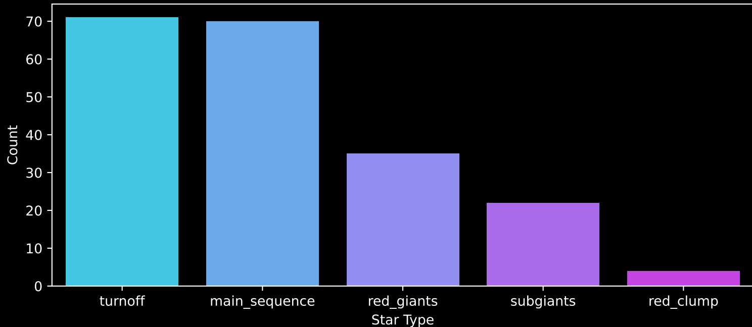
GALAH DR4 Field: [7239] Count plot of Star Type
