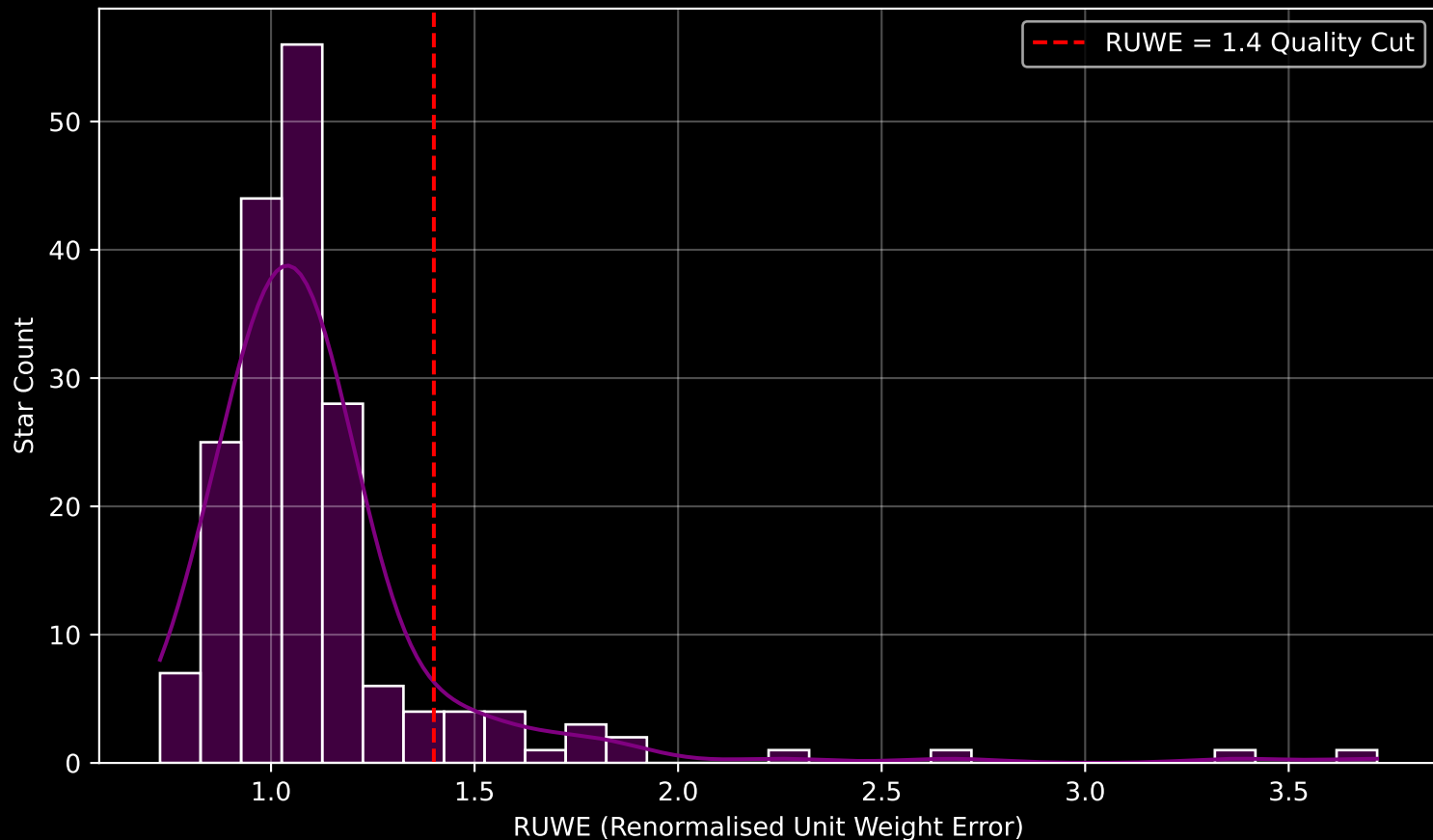
GALAH DR4 Field [7239] RUWE Distribution (n= 188)
