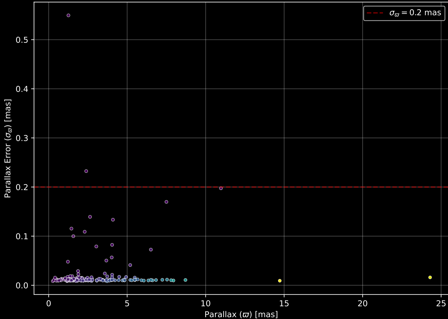
GALAH DR4 Field: [7239] Parallax Quality (n= 202)
