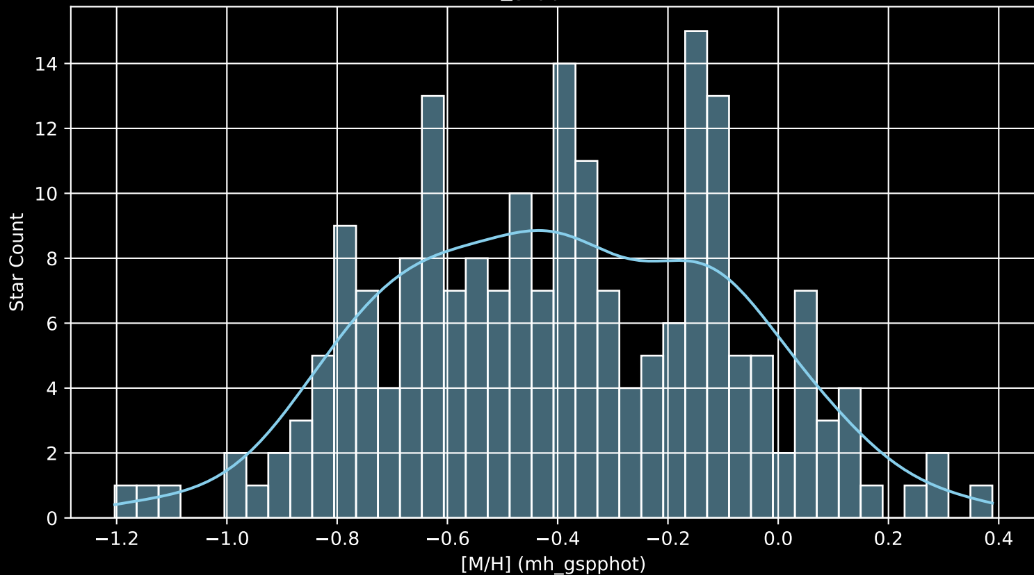
GALAH DR4 Field: [7239] [M/H] (mh_gspphot) (n= 202)
