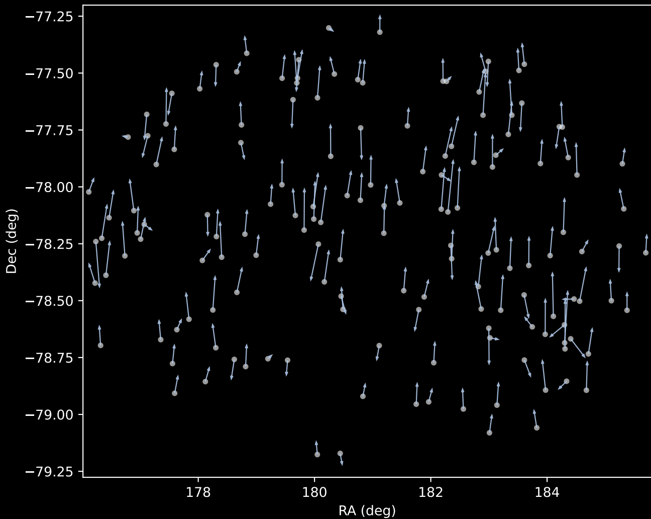
GALAH DR4 Cluster 1 Proper Motion Vectors (n=151)
