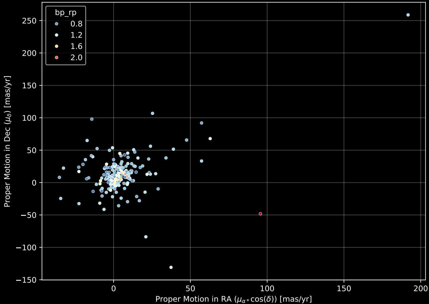
GALAH DR4 Field: [7239] Proper Motion Diagram (n= 202)
